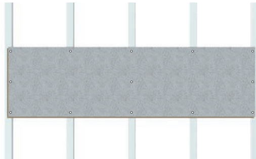
④ Screw pattern for panel widths of 600 mm and 850 mm
